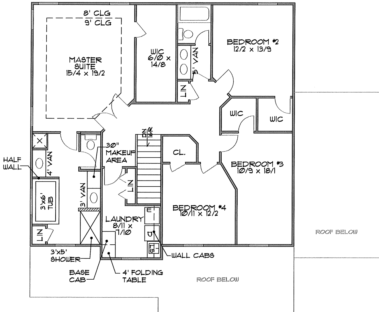
COBBLESTONE SECOND FLOOR PLAN
